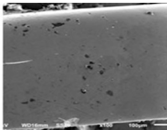
Figure 2. Bracket surfaces after 4 months of use. Discernible small pits of corrosion. SEM image 100 x
