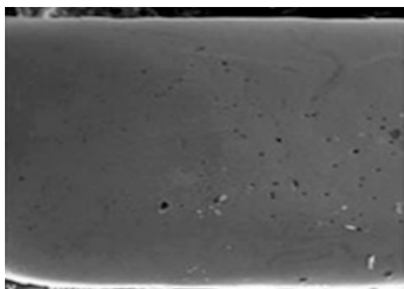
Figure 1. Bracket surfaces from control group (before treatment). No sign of corrosion. Visible only machining defects as scattered dots. SEM image 100 x.
