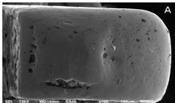
Figure 3. Bracket surfaces after 8 months of use. Discernible more numerous cavities of corrosion. SEM image 100 x.
