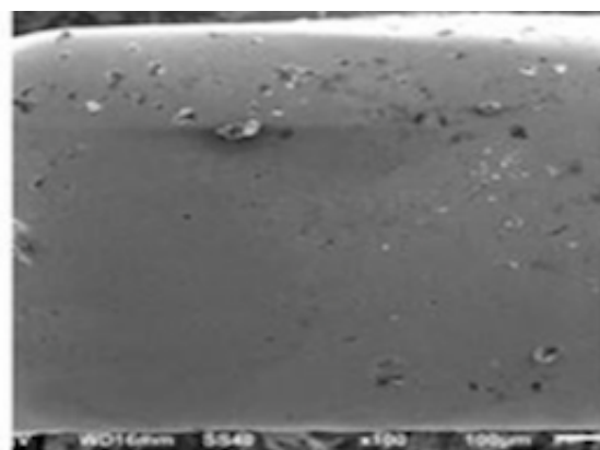
Figure 1. Bracket surfaces from control group (before treatment). No sign of corrosion. Visible only machining defects as scattered dots. SEM image 100 x.
