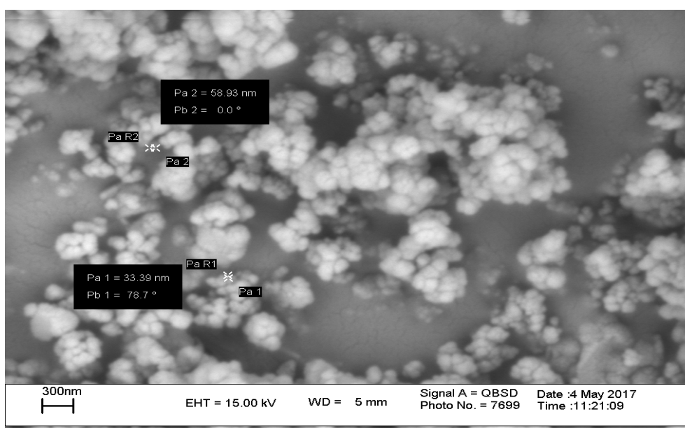
Figure 1. Scanning electron microscope micrograph of potassium silicate nanoparticles
