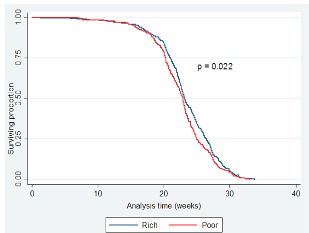
Figure 2: Kaplan – Meier curve of surviving proportion of preterm delivery based on socioeconomic status
