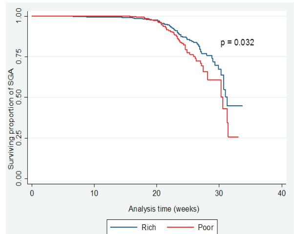
Figure 1: Kaplan – Meier curve of surviving proportion of Small for Gestational Age based on socioeconomic status
